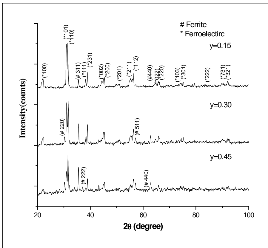
Fig. 1. X-ray diffraction patterns of y(\text{Ni}_{0.5}\text{Cu}_{0.2}\text{Zn}_{0.3}\text{Fe}_2\text{O}_4) + (1-y) (50% \text{BaTiO}_3 + 50% PZT) ME composites
