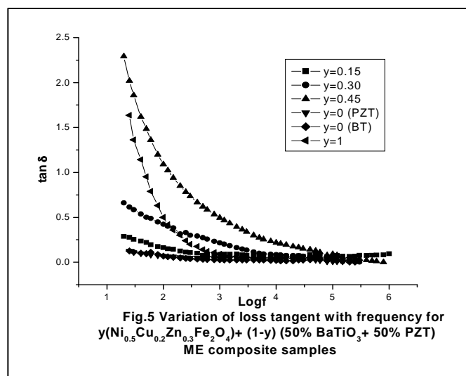
Fig. 5 shows variation of loss tangent with frequency. The variation of \text{Tan } \delta with frequency shows the similar nature as that of \epsilon with frequency
