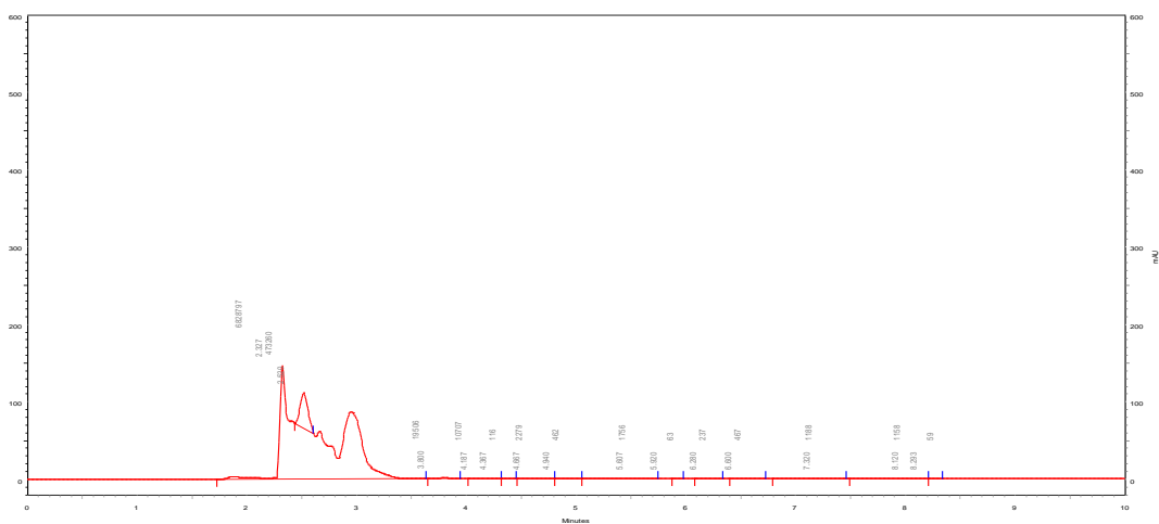
Figure 7. Thermal degradation of APR
