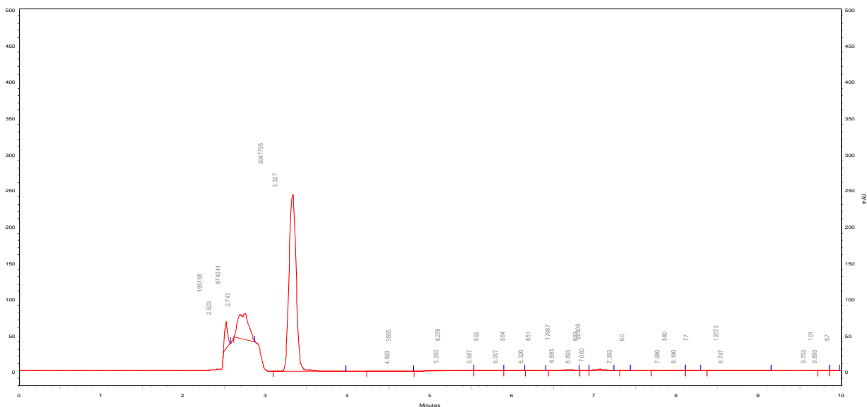
Figure 4. Acid degradation of APR
