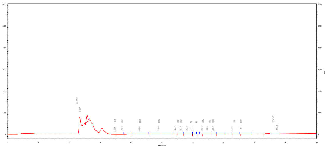
Figure 8: UV light degradation of APR
