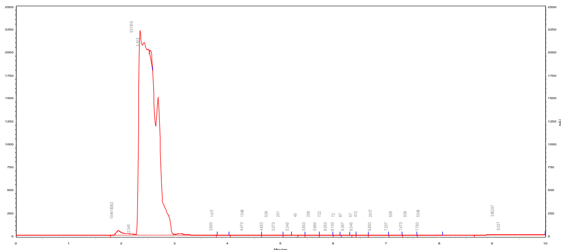
Figure 6: Oxidative degradation of APR
