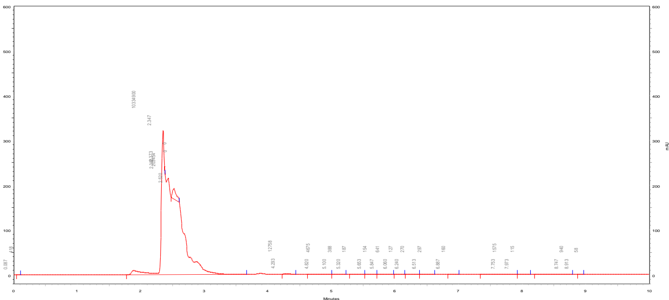
Figure 5 Alkali degradation of APR
