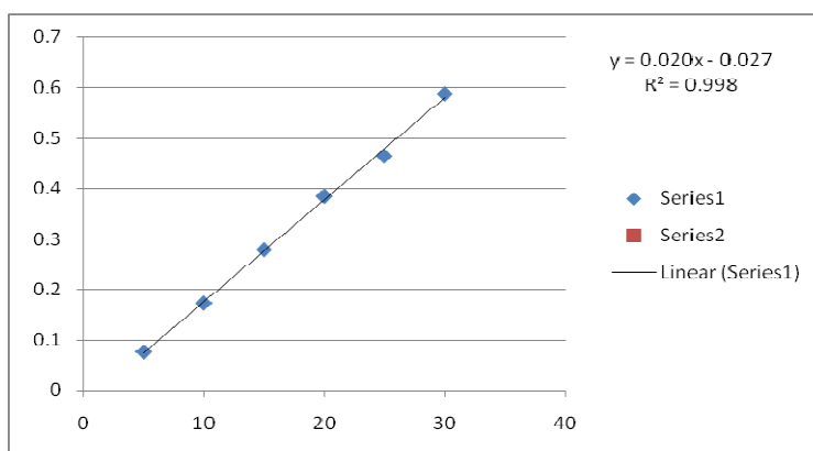
Fig(1) Linearity of ibuprofen
