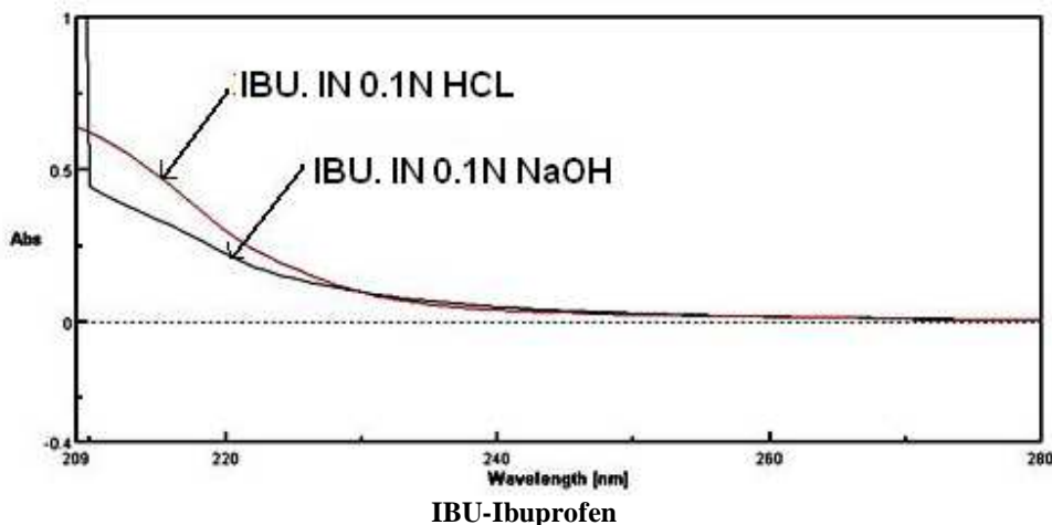
Fig. 4: Overlain spectra of Ibuprofen in 0.1 N HCL and 0.1 NaOH
