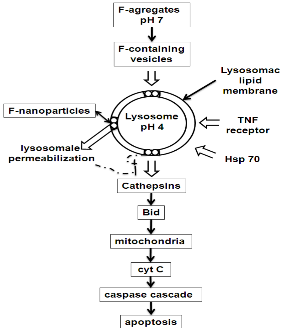
Fig.5. The effect of C_{60}(C(COOH)_2)_2 on lysosomal and mitochondrial apoptotic pathway, according [158].
