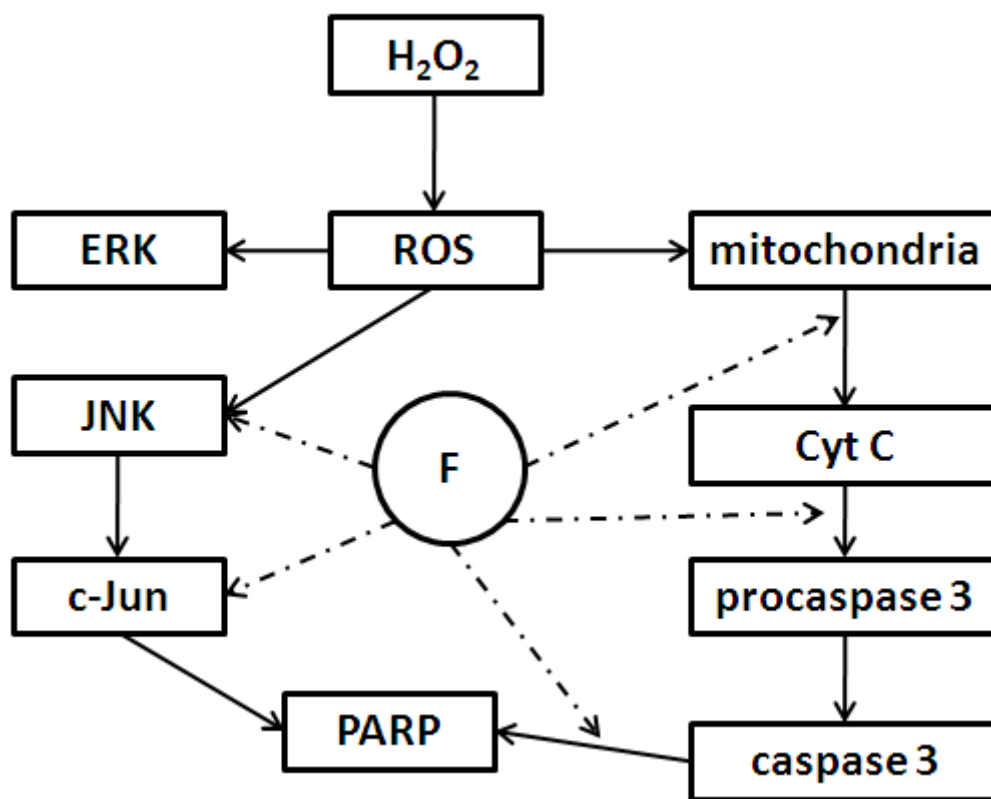
Fig.4. A scheme of events in CMECs, according to [119], induced by hydrogen peroxide and treatment by C 60 (C(COOH) 2 ) 2 nanoparticles. Changes are mediated by decreasing of JNK phosphorylation and inhibition of ROS production. There is down-regulation of the signaling pathway with decreasing of c-Jun and caspase-3 activation and inhibition of PARP cleavage and release of a mitochondrial cytochrome C.
