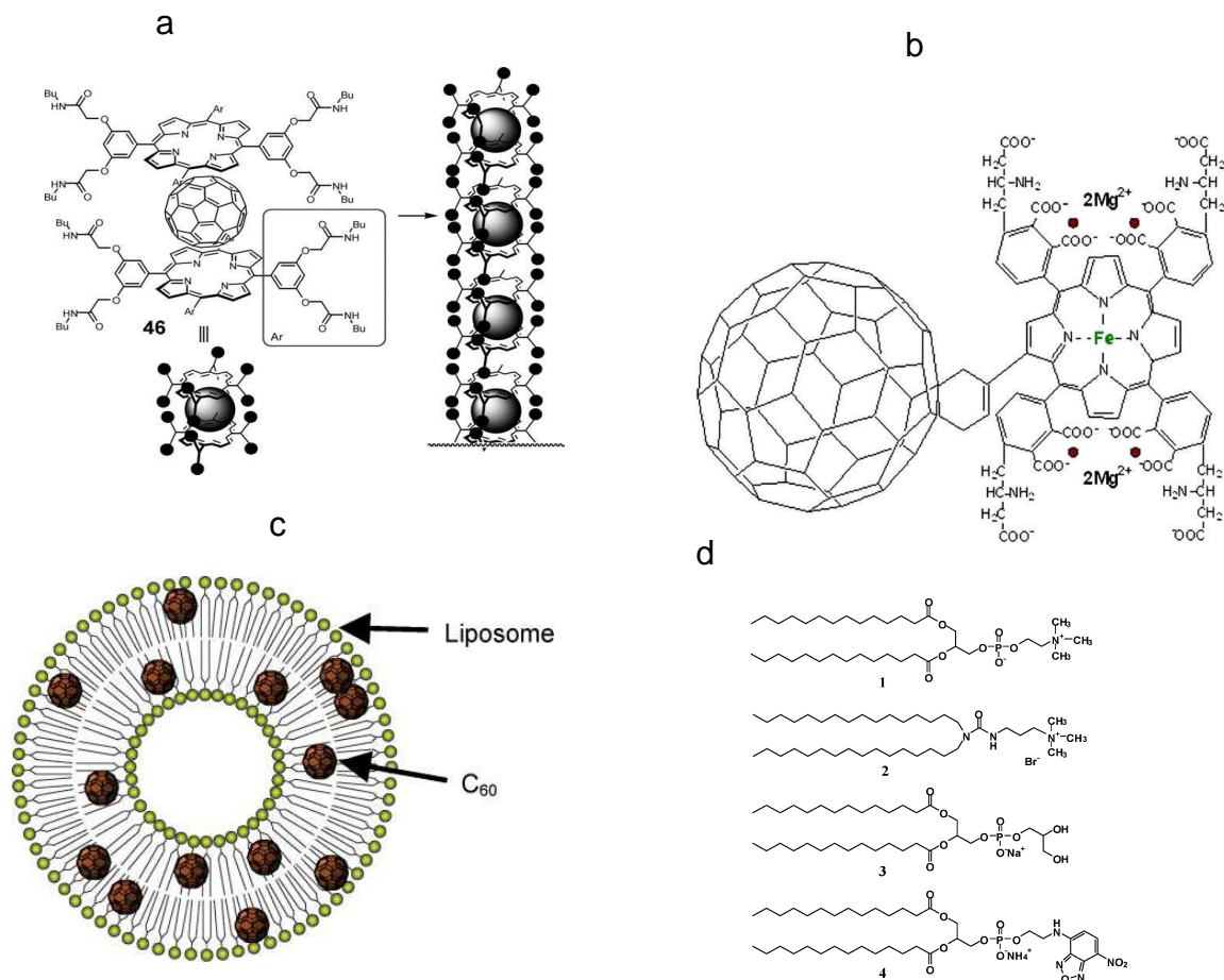
Fig.7. (a)- Structure of supramolecular aggregate, octaamidoporphyrin with fullerene C 60 . (b)-bakminsterfullerene (C 60 ) – 2 – (butadiene – 1- yl) tetra (o – γ – amino butyryl–o-phthalyl) ferroporphyrin (PMC16), containing 4 ions of magnetic isotope of 25 Mg, (c)- Complex of C 60 with a liposome, possessing, due to compounds 1-4 (d), different surface charge, according to [258].
