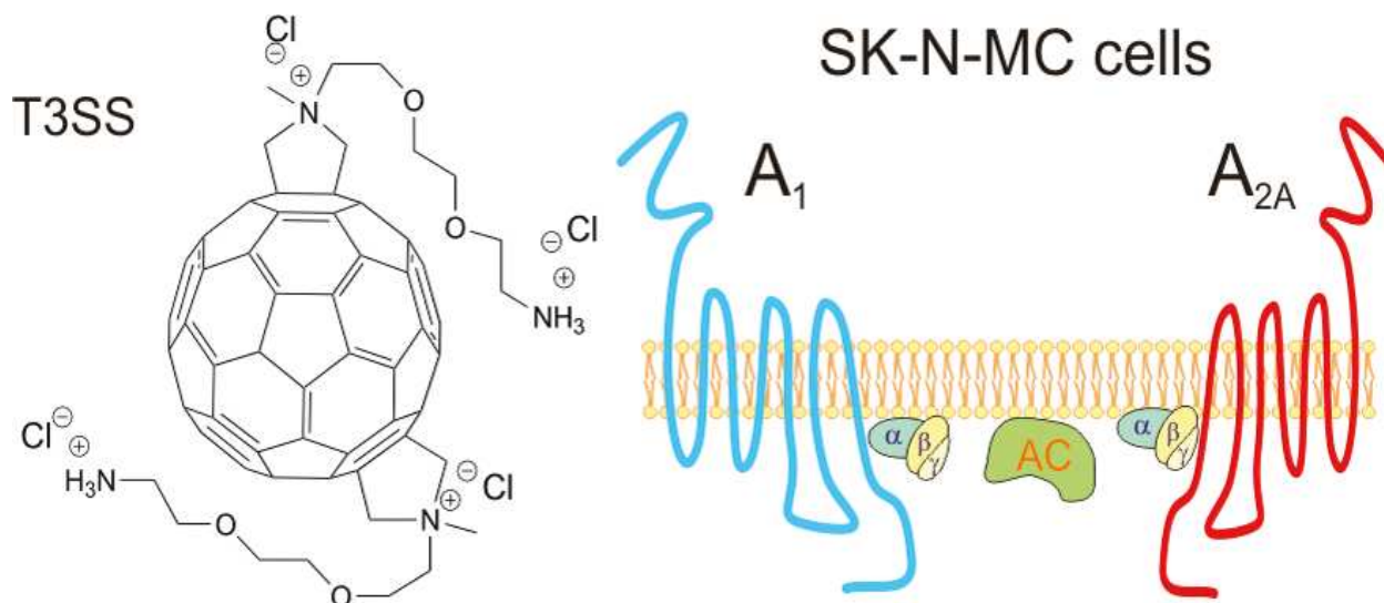
Fig.3. C 60 -derivative and adenosine receptors in SK-N-MC cell line of human neuroepithelioma. Copy from [88].
