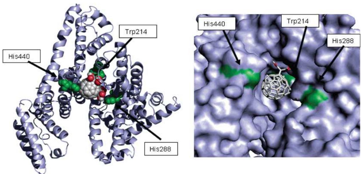
Fig.6. A site of carboxyfullerene binding with HSA, predicted by docking. Copy from [195].
