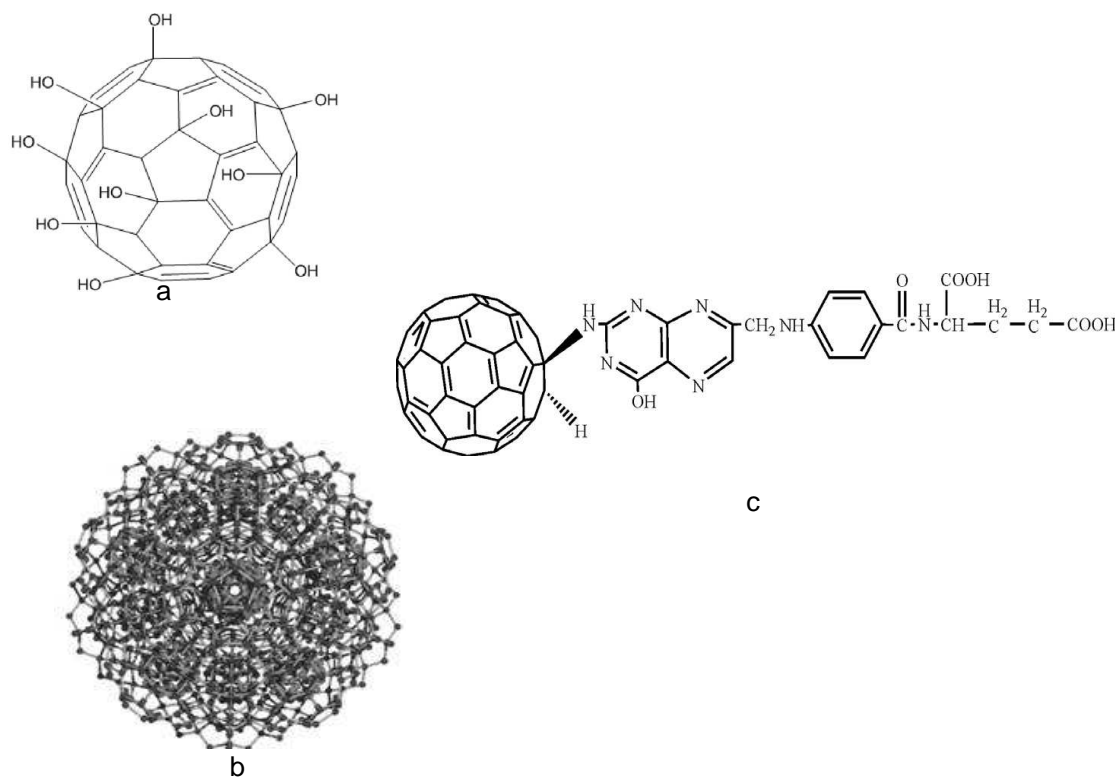
Fig.1. Hydroxylated fullerene (a), spheric cluster (C 60 @{H 2 O} n ) m (b), C 60 -folic acid (c).
