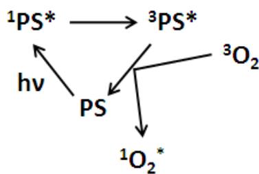
Fig.2. Mechanisms of singlet oxygen and superoxide radical generation by fullerenes.
