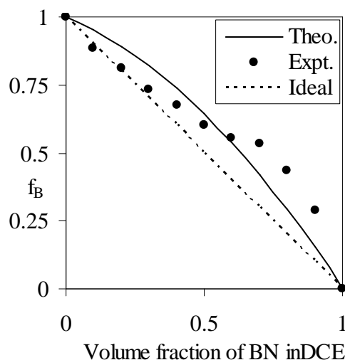
Figure 2. The Bruggeman plot for BN-DCE mixture at 35°C. Dashed line denote original model (equation 6).
