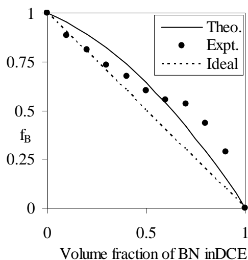
Figure 2. The Bruggeman plot for BN-DCE mixture at 35°C.
