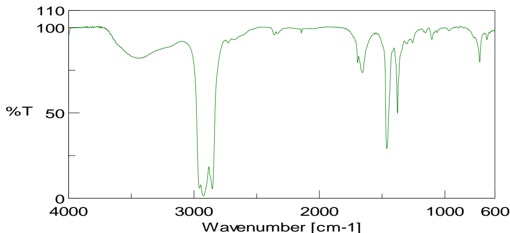
Figure 2. IR spectrum of compound 7.
