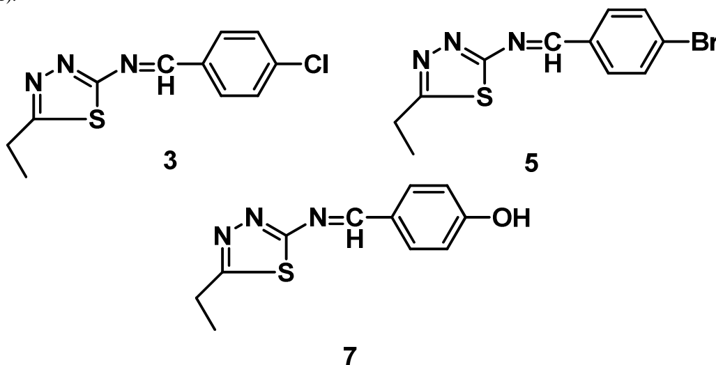
Figure 1. Structures of Schiff base ligands.
