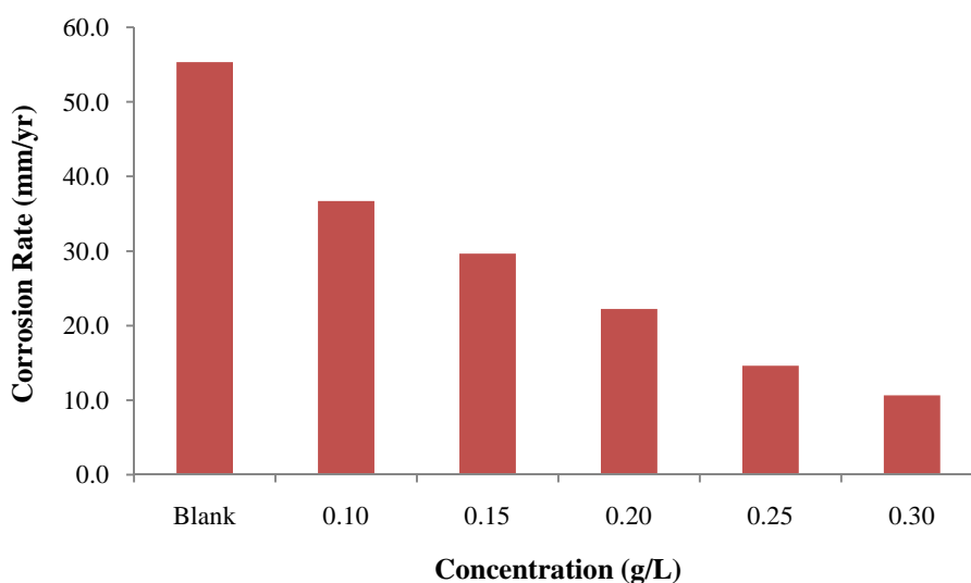
Figure i. Corrosion rates of aluminium alloy AA8011 in various concentrations of Euphorbia hirta
