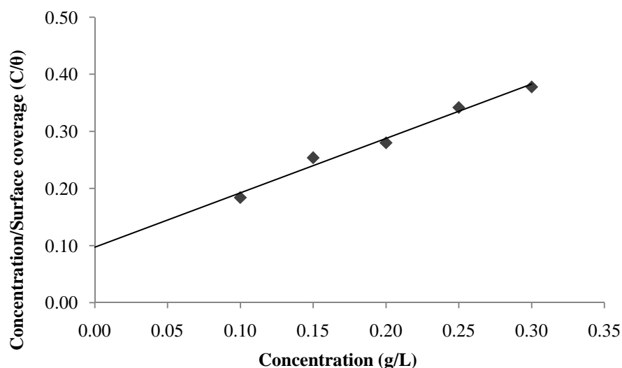
Figure iii. Langmuir isotherm for Euphorbia hirta adsorption on AA8011 aluminium alloy in 0.5M HCl
