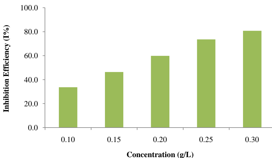
Figure ii. Inhibition efficiency of various concentrations Euphorbia hirta extract on aluminium alloy
