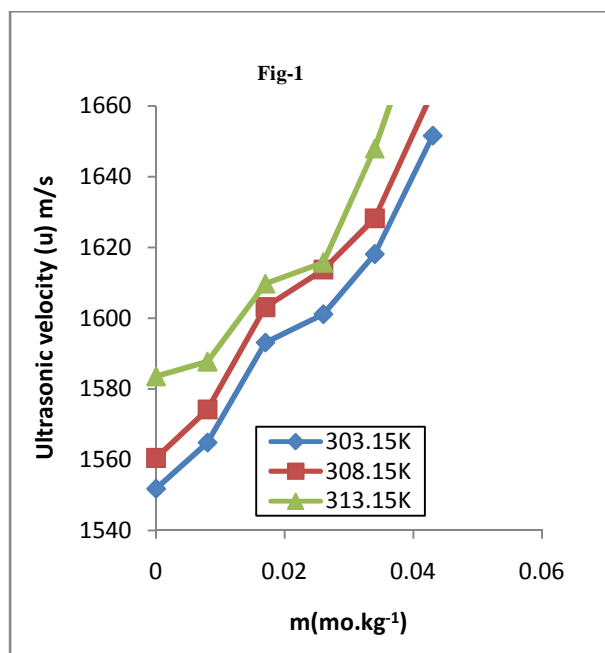
Fig-1- Plot of ultrasonic velocity (u) against mole fraction (m) for the system (water + NaCl + serine) at 2MHz and at 303.15, 308.15 and 313.15K temperatures
